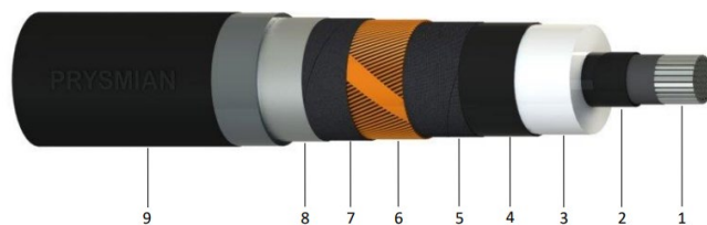
HV2 diagram
