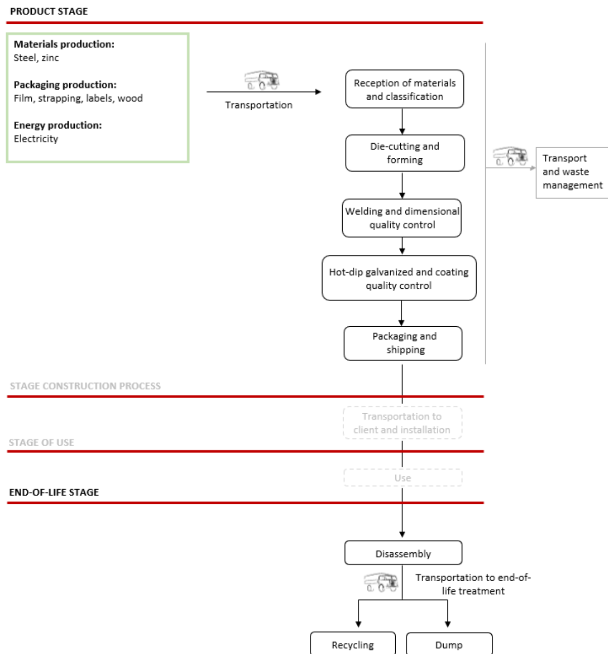
Image 1 Production process diagram.
